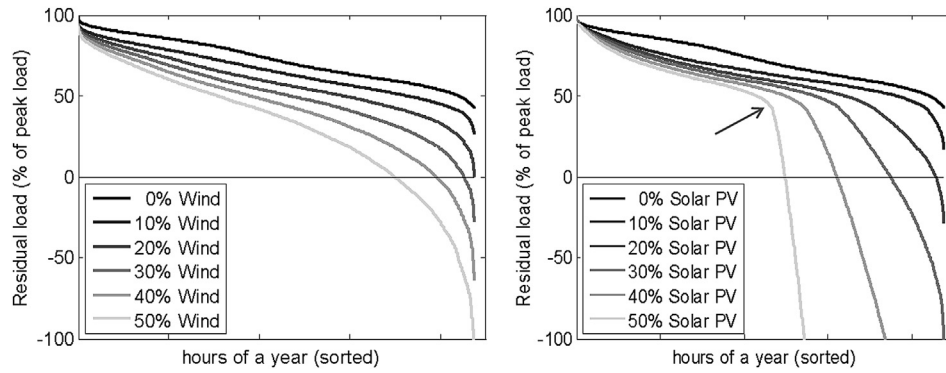
Fig. 5. Residual load duration curves (RLDC) for increasing shares of wind (left) and solar PV (right) in Germany. With higher shares the RLDC continuously become steeper. Wind generation slightly covers peak load but increasingly contributes to intermediate and base load as well as to overproduction. Solar PV does not reduce peak capacity requirements. It covers intermediate load at low shares. With higher shares (>10%) additional solar generation mostly contributes to base load and overproduction.
