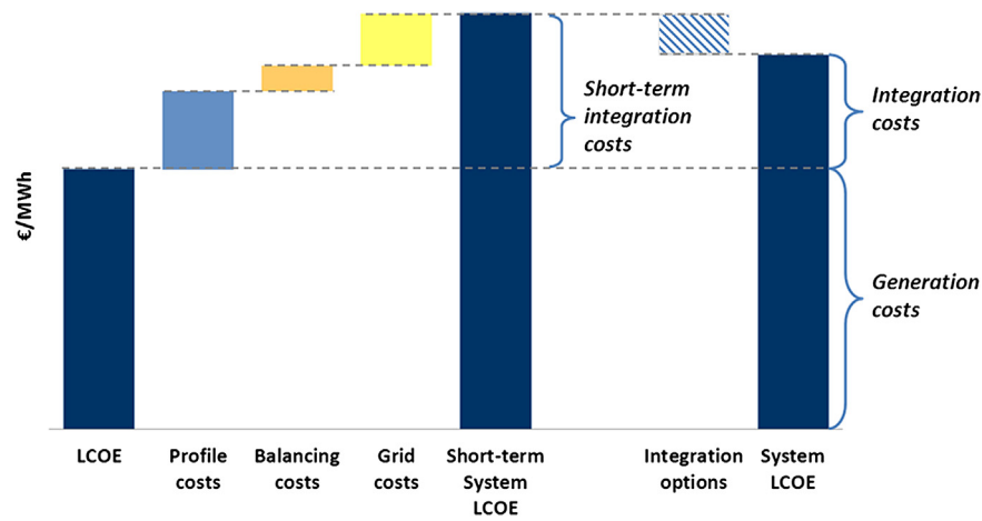
Fig. 6. Integration costs are divided into three components: profile, balancing and grid costs. To some extent integration costs that occur in the short term can be reduced by integration options in the long term.
