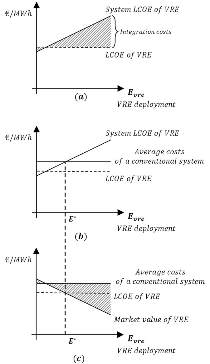
Fig. 2. (a) System LCOE are the sum of LCOE and marginal integration costs (per MWh) while integration costs increase with VRE penetration. An optimal quantity E^* of VRE can be derived from (b) System LCOE or equivalently (c) the market value of VRE.
