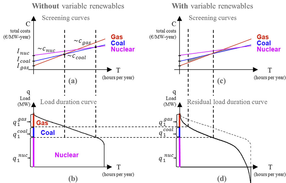
Fig. 8. (Illustrative): Optimal long-term capacities are derived without VRE (a, b). With VRE the LDC transforms to an RLDC (d). In the short-term perspective the capacities remain unchanged (b, d). Hence, specific costs increase because technologies operate in full-load hour ranges where they would not be cost-efficient if capacities could optimally adjust (c).
