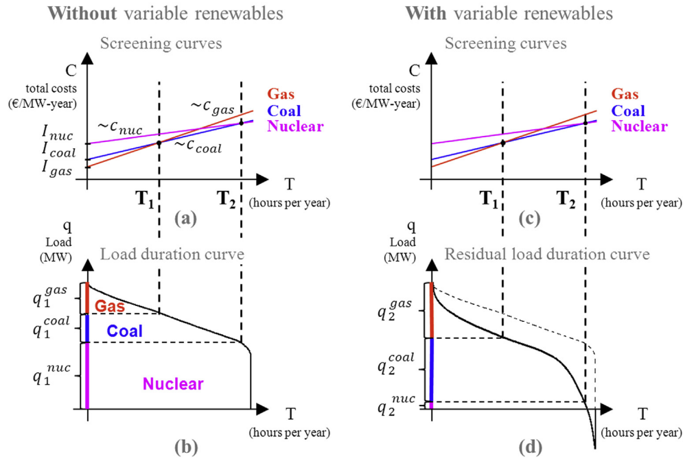
Fig. 7. (Illustrative): Long-term screening curves and load duration curves without (left) and with wind deployment (right). Wind changes the residual load duration curve (c, d). Thus capacities adjust towards lower fixed-to-variable-costs ratio (more gas capacity, less nuclear capacity).
