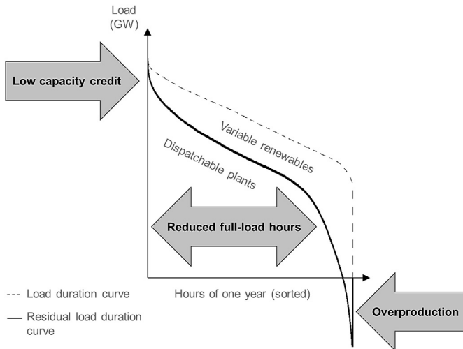
Fig. 4. (Illustrative): Residual load duration curves capture three main challenges of integrating VRE. While hardly any generation capacity can be replaced due to their low capacity credit, the full-load hours of conventional plants are reduced. At higher shares VRE supply exceeds load and thus cannot directly be used.
