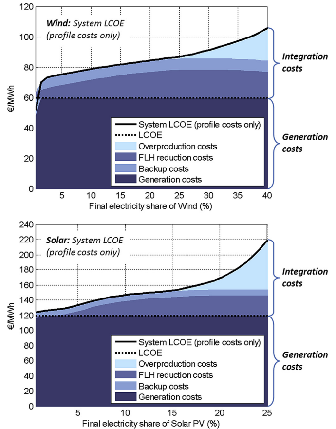
Fig. 10. System LCOE (profile costs only) for increasing generation shares of wind (above) and solar PV (below) for Germany estimated with a power system model that is designed for calculating profile costs. These costs are decomposed into three cost drivers. The full-load hour (FLH) reduction of conventional plants is the largest cost driver at moderate shares, while overproduction costs significantly increase integration costs at high shares.
