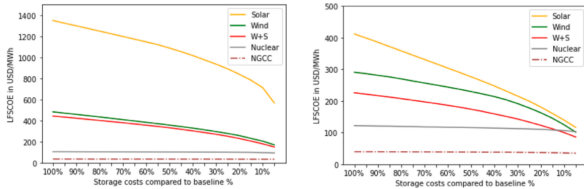
Fig. 3. LFSCOE with decreasing capacity costs for storage. Development of LFSCOE if storage costs decrease significantly for the market in Germany (left) and Texas (right).
