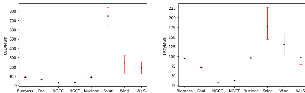
Fig. 5. LFSCOE95 Mean and Variance in the German (left) and ERCOT market.
