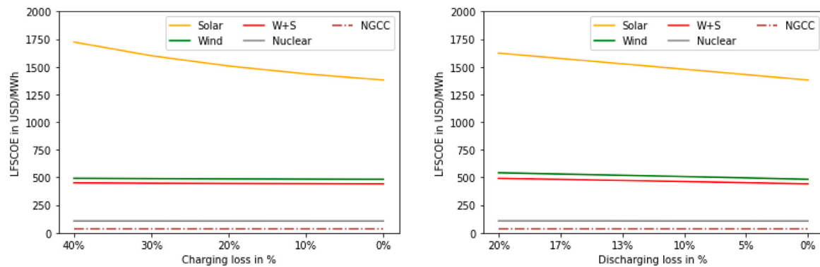
Fig. 4. LFSCOE with charging and discharging losses.
