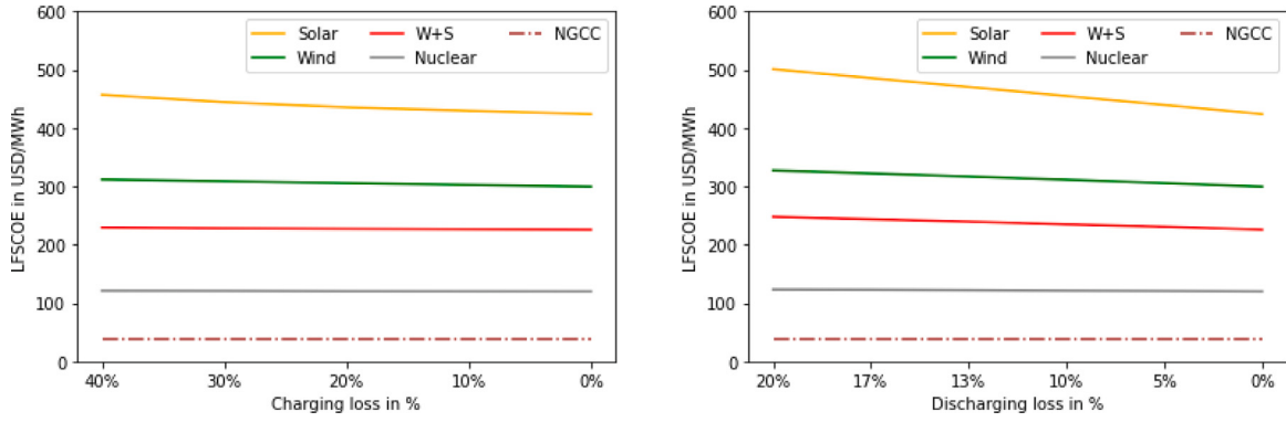
Fig. 7. LFSCOE with charging and discharging losses in Texas.
